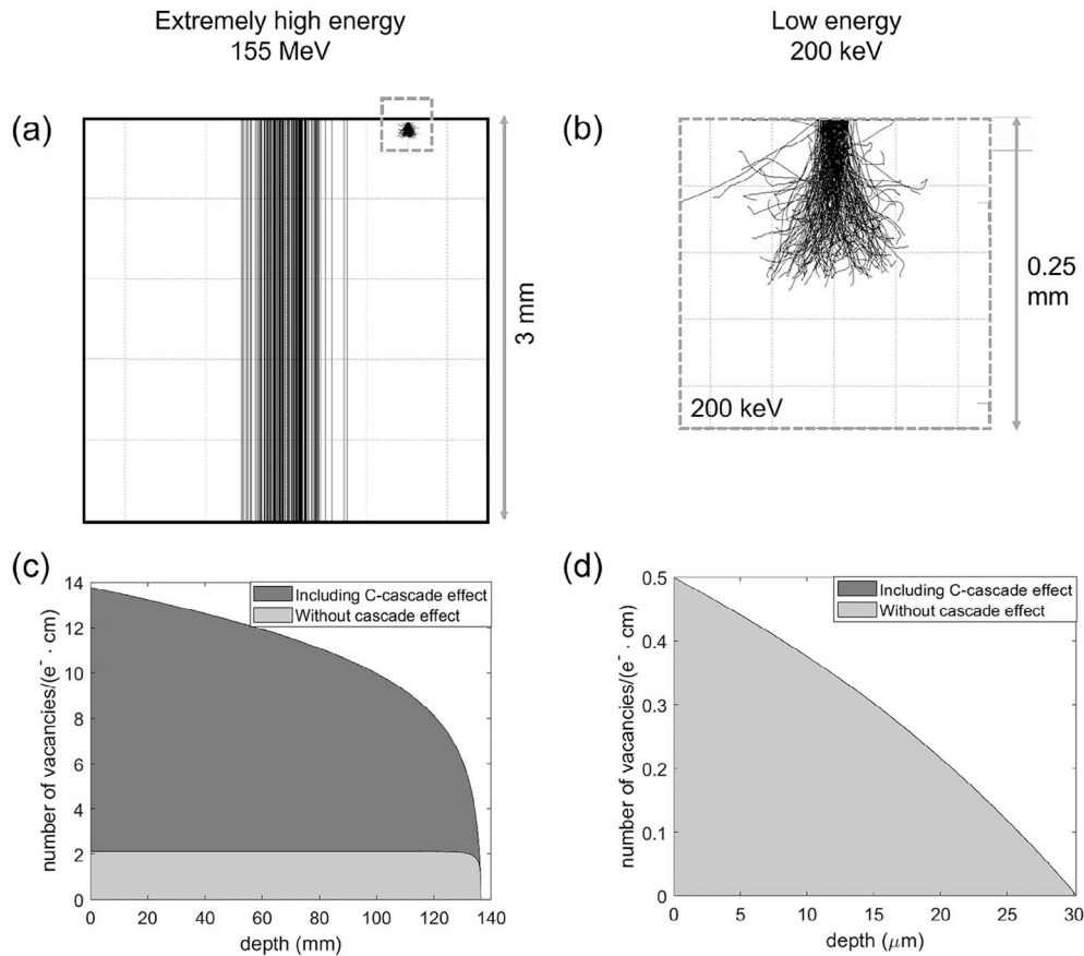
Figure 1. a,b) Trajectories of 200 electrons in diamond, simulated using CASINO software. a) 155 MeV electron irradiation, 500 \mu\text{m} beam diameter. b) 200 keV electron irradiation, 15 \mu\text{m} beam diameter. c,d) Simulation of the number of vacancies per centimeter depth generated by 1 accelerated electron at c) 155 MeV energy and d) 200 keV energy. The contribution of the initial recoiled atoms (filled light gray) and the secondary cascade process (filled dark gray) are highlighted. Note the different axes limits in the two cases.
